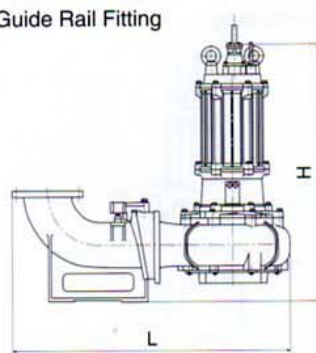
Guide Rail Fitting
