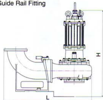
Guide Rail Fitting
